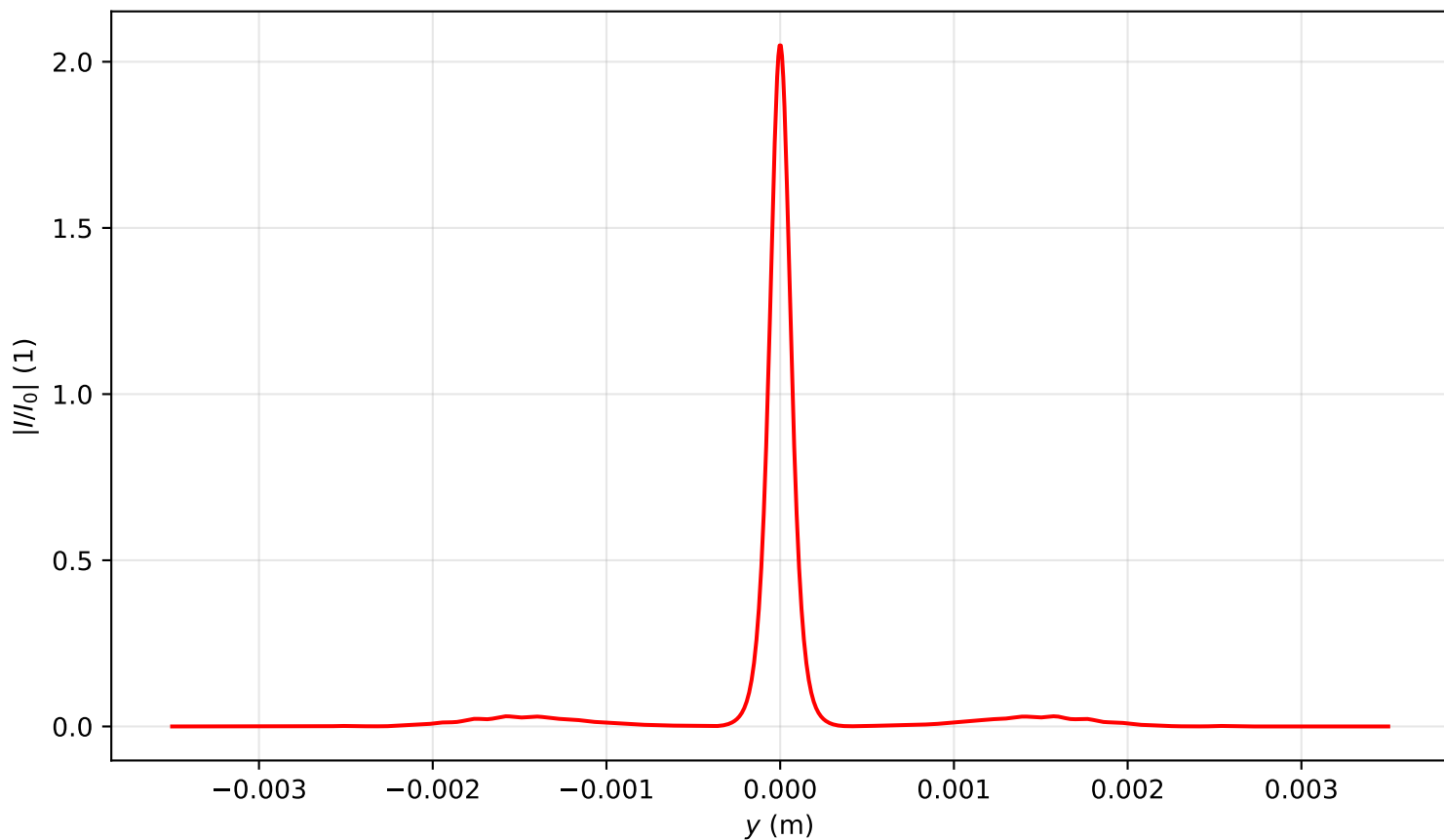
Intensity profile I(x = 0, y, z = 1.274)/I_0 , \text{Pin}=8.0\text{Pcr} , artificial time
